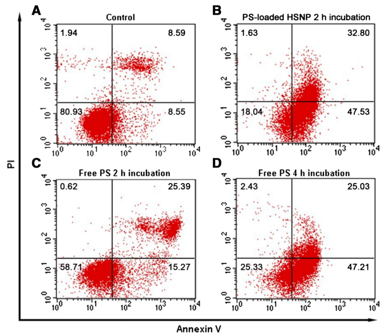
Figure 2 Flow cytometry analyses of groups A, B, C, and D. Group A cells are the blank control; group B cells were treated with 5 mg/L nanoscale Photosan for 2 h at 5 J/cm 2 ; group C, cells received 5 mg/L conventional Photosan for 2 h at 5 J/cm 2 ; group D cells were treated with 10 mg/L conventional Photosan for 4 h at 10 J/cm 2 . Lower left quadrants represent normal cells; lower right quadrants are early apoptotic cells; upper right quadrants represent late, dead apoptotic cells; upper left quadrants are mechanically damaged cells. The apoptotic rate was defined as 100* (sum of early apoptotic and late apoptotic cells)/total number of cells.
