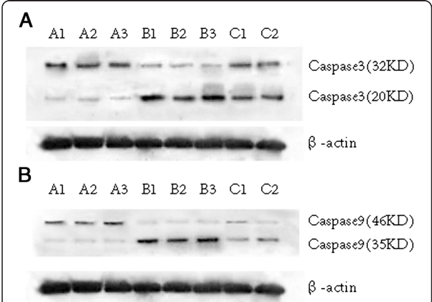
Figure 3 Active caspase-3 (A) and caspase-9 (B) protein levels in cancer cells after conventional and nanoscale photosensitizer PDT. A1, A2, and A3: blank control samples; B1, B2, and B3: nanoscale Photosan-treated samples; C1 and C2: Photosan-treated samples.
