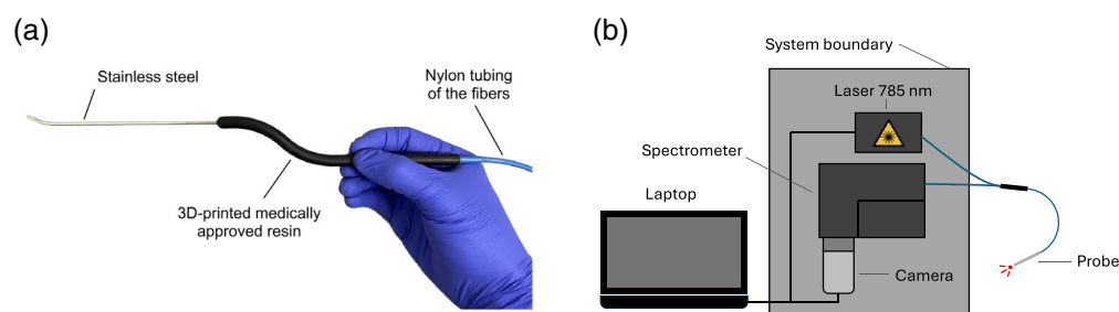
Fig. 1 (a) Handheld endonasal Raman spectroscopy probe. Annotations indicate the different types of sterilizable materials used to fabricate the device. (b) Schematics of the complete system illustrating the enclosed module housing the near-infrared laser, the spectrometer, and the sensor, all connected to the endonasal probe. A control laptop manages all system operations.
