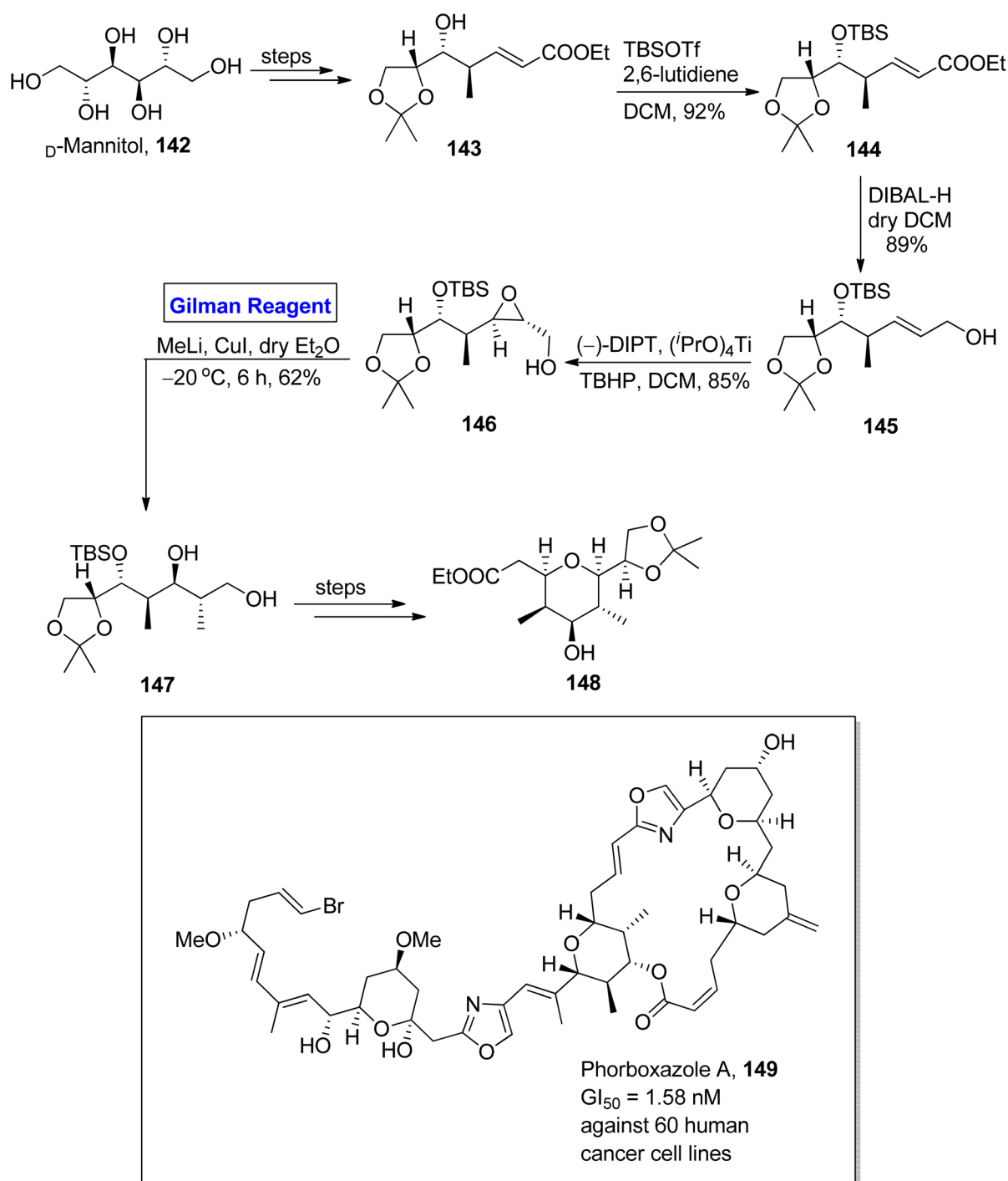
Scheme 16 Synthesis of the C20–C27 fragment 148 of phorboxazole A.
