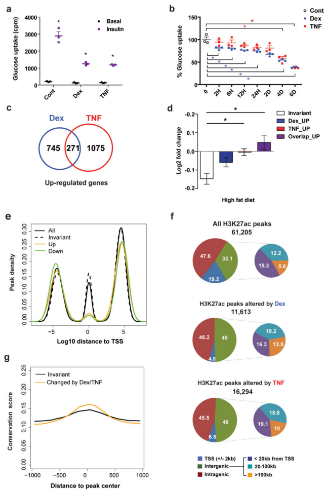
Figure 1. Transcriptional and epigenomic profiling of the insulin resistance model a , Basal and insulin-stimulated glucose uptake in cells treated with Dex and TNF for 6 days ( n=3 independent experiments, each point represents the mean of 6 independent replicates p<0.05 by Student's t-test, mean \pm SEM). b , Adipocytes were treated with Dex or TNF for the indicated lengths of time and the development of insulin resistance was monitored by glucose uptake assay; results are expressed as percent of glucose uptake remaining compared to untreated (control) ( n=3 independent experiments, each point represents the mean of 6 independent replicates p<0.05 by Student's t-test, mean \pm SEM). c , Venn diagram depicting the number of up-regulated genes in response to Dex and TNF treatment. These numbers represent a 'unity' set in which all time points were combined. d , Fold change (log 2 scale) of genes from c in the white adipose tissue of obese vs. lean mice 22 , n = number of genes in each group (invariant = 160, Dex UP = 357, TNF_UP = 512, Overlap_UP = 110) p<0.05 by Student's t-test, mean \pm SD). e , H3K27ac peak density as a function of distance to the TSS of the nearest gene. f , Distribution of all H3K27ac peaks in untreated cells (top), and the distribution of H3K27ac peaks that change with Dex (middle) and TNF are shown (bottom). g , Sequence conservation score of DNA under distal H3K27ac peaks (>10 kb from TSS) as a function of distance from peak center, for invariant and changed peaks.
