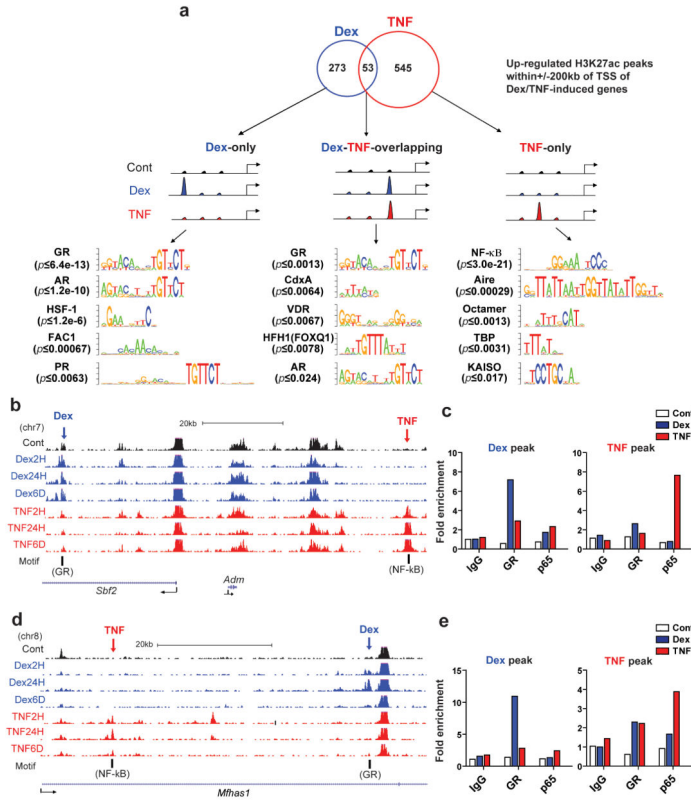
Figure 2. Motif analysis of co-induced H3K27ac enhancer peaks a , Venn diagram depicting H3K27ac peaks up-regulated by Dex and TNF within \pm 200 kb of the TSS of an induced gene. Also depicted are significantly enriched binding sites with TRANSFAC position weight matrix results recovered by motif analysis of ‘Dex only’, ‘TNF-only’, and ‘Dex-TNF overlapping’ peaks (with p values determined by Fisher’s Exact test). b , Tracks from an up-regulated gene ( Sbf2 ) showing distinct Dex- and TNF-sensitive H3K27ac peaks. c , ChIP-PCR results from the Dex- and TNF-induced peaks depicted in b (data represent mean of n = 3 dishes, data from 2 additional independent experiments shown in Source Data Table), using anti-GR, anti-p65, or IgG. d , Tracks from an up-regulated gene ( Mfhas1 ) showing ‘Dex-TNF-nonoverlapping’ H3K27ac peaks. e , ChIP-PCR results from the ‘Dex-only’ and ‘TNF-only’ peaks depicted in d (data represent mean of n = 3 dishes, data from 2 additional independent experiments shown in Source Data Table).
