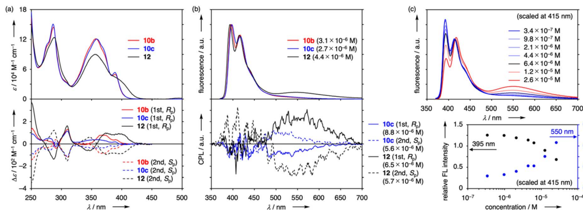
Fig. 2 (a) UV/vis absorption (top) and CD (bottom) spectra of 10b , 10c and 12 in \text{CHCl}_3 . (b) Fluorescence (top, \lambda_{\text{ex}} = 350 \text{ nm} ) and CPL (bottom, \lambda_{\text{ex}} = 280 \text{ nm} ) spectra of 10b , 10c and 12 in \text{CHCl}_3 . (c) Concentration-dependent fluorescence spectra of 12 in \text{CHCl}_3 (top) and relative intensity plot (bottom) of peaks at 395 nm (black, left axis) and 550 nm (blue, right axis) scaled at 415 nm.
