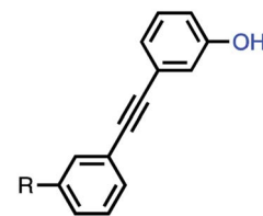
Fig. 13 Phenol 1-mer (R = S -β-citronelloxy).
