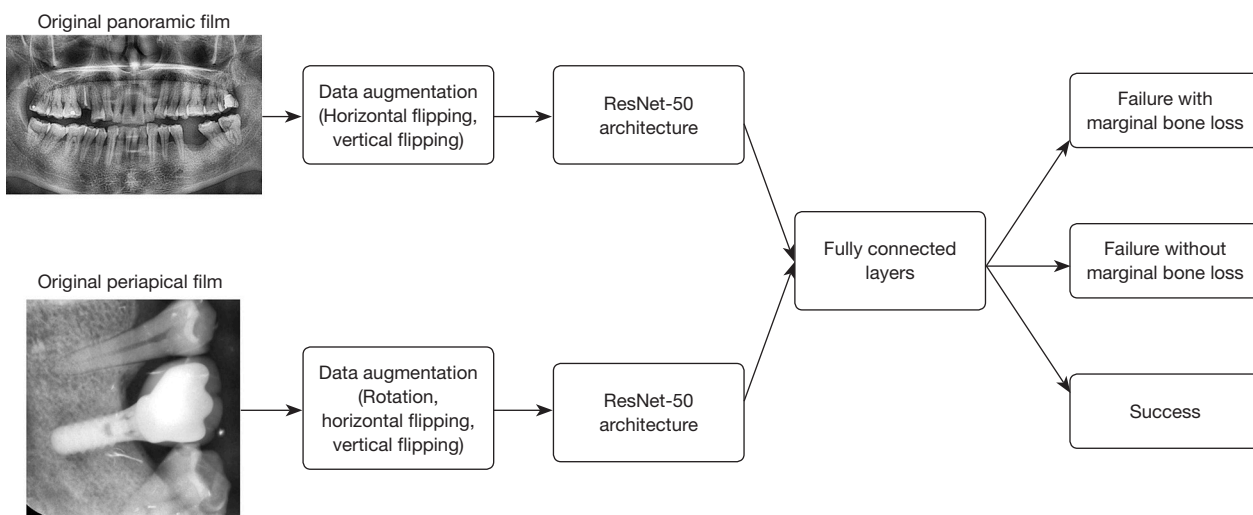
Figure 4 Architecture of the deep convolutional neural network model. ResNet-50 architecture: a pretrained deep CNN with 50 deep layers. CNN, convolutional neural network.
