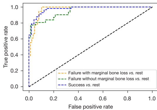
Figure 6 Multiclass ROC curve comparison for classification in implant outcomes. ROC, receiver operating characteristic.
