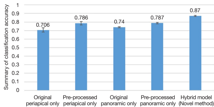
Figure 5 Classification accuracy of hybrid model compared to other four methods. Hybrid model: both periapical and panoramic images were used.
