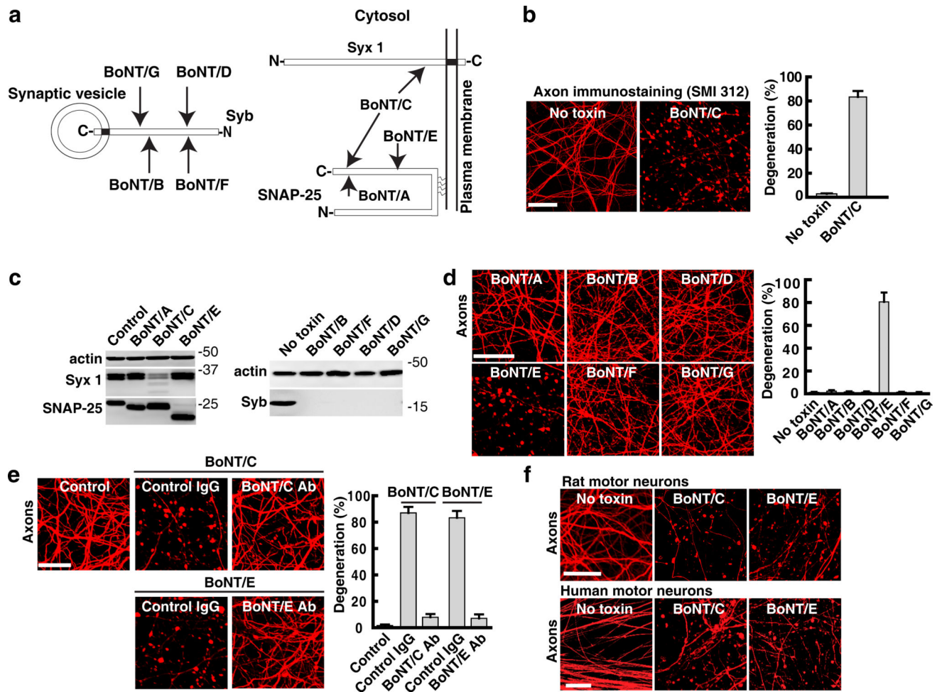
Figure 1. BoNT/C and E can induce degeneration of cultured rodent and human neurons (a) Schematic drawings of the cleavage sites on neuronal SNAREs for the seven BoNTs. BoNT/B, D, F, and G cleave Syb. BoNT/A and E cleave SNAP-25. BoNT/C cleaves both Syx 1 and SNAP-25.
