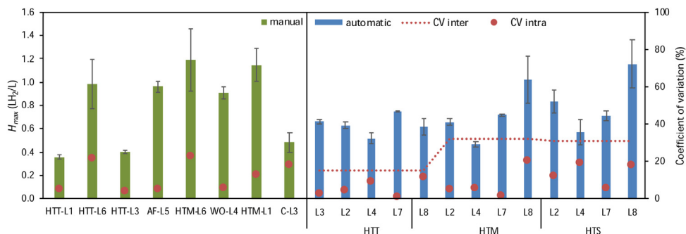
Fig. 7. Cumulative hydrogen production ( H_{max} ) specific to the working volume ( L H_2 L^{-1} ), for the manual and automatic protocols, and its corresponding intra- and inter-laboratory variation. For the manual protocol evaluation different inoculum were tested by different laboratories, meanwhile for the automatic protocol three different source of inoculum were evaluated in different laboratories. The different inoculum sources were heat-treated anaerobic sludge from a thermophilic digester (HTT); heat-treated anaerobic sludge from a mesophilic digester (HTM); biomass from an auto-fermented effluent rich in sucrose (AF); aerobic sludge pretreated by cell wash-out (WO); compost from kitchen wastes (C); and heat-treated anaerobic sludge from a digester treating solid wastes (HTS). L1–L8 stands for results from different laboratories.
