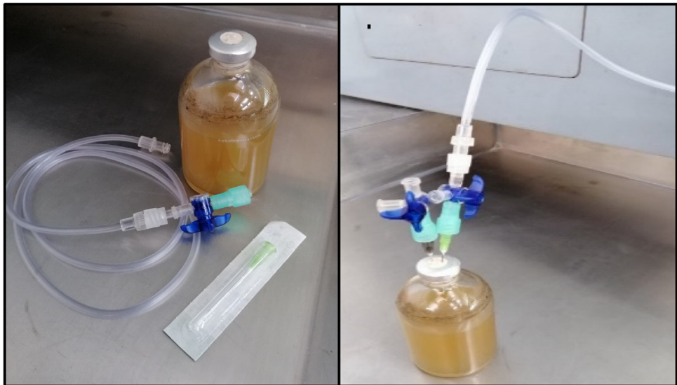
Fig. 3. Headspace exchange on the serum bottles.
