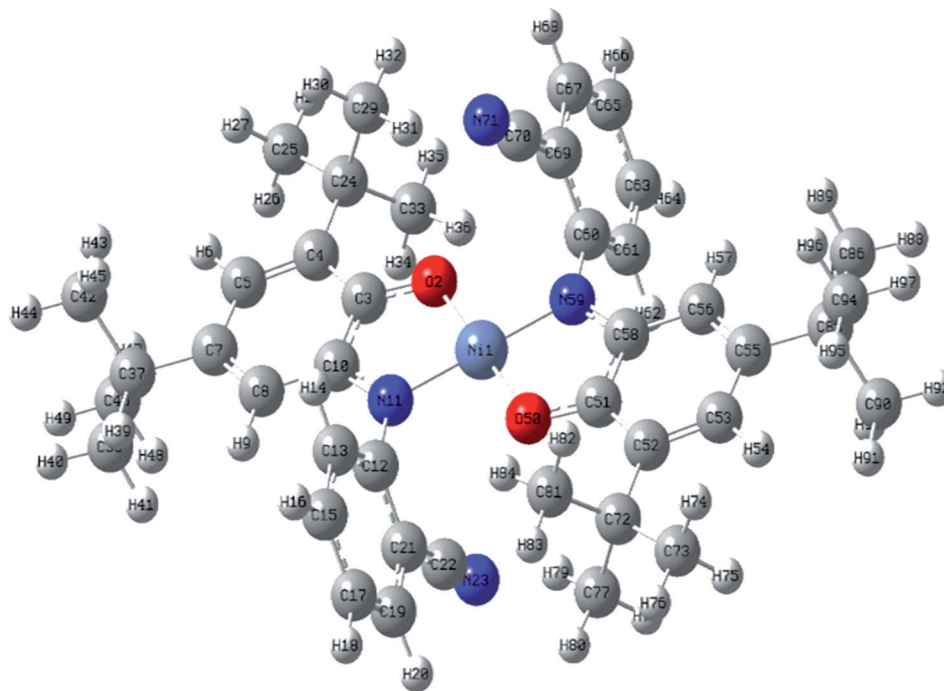
Fig. 5 The Optimized structure of catalyst, \text{Ni}^{\text{II}}\text{L}_2^{\text{NIS}} . Selected bond lengths [ \text{\AA} ] and angles [ ^\circ ]: Ni(1)–O(2) 1.83, Ni(1)–N(11) 1.84, C(3)–C(4) 1.43, C(4)–C(5) 1.38, C(7)–C(8) 1.38, C(8)–C(10) 1.42, O(2)–C(3) 1.30, C(10)–N(11) 1.35, C(21)–C(22) 1.44, C(22)–N(23) 1.16, O(2)–Ni(1)–O(50) 180.0, O(2)–Ni(1)–N(11) 85.75, O(50)–Ni(1)–N(11) 94.25, C(3)–O(2)–Ni(1) 113.75.
