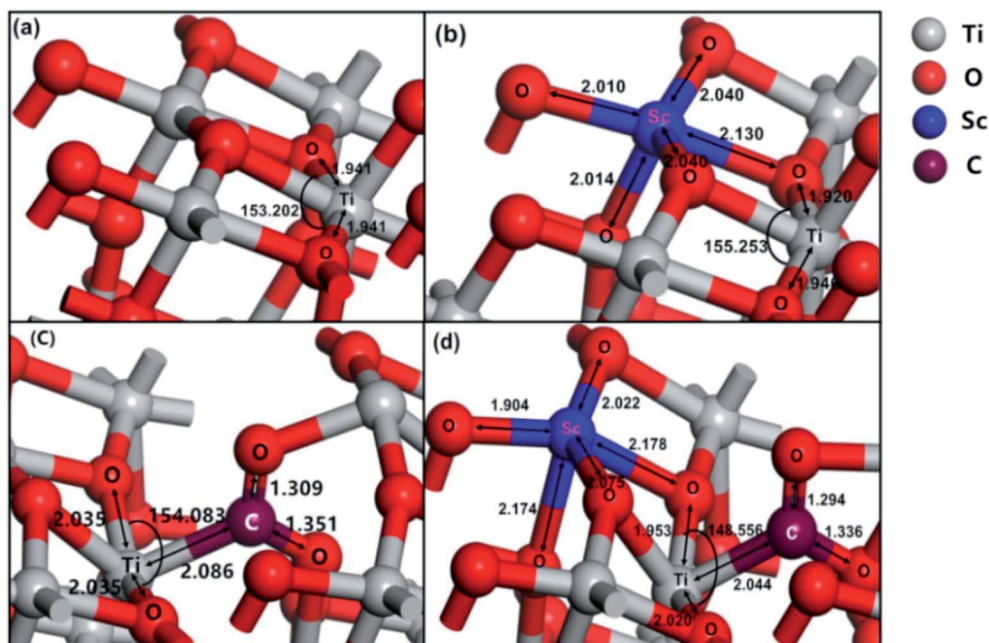
Fig. 2 Optimized geometrical configurations and partial bonds length for (a) pure, (b) Sc-doped, (c) C-doped, and (d) Sc/C-codoped TiO 2 (101) surfaces.
