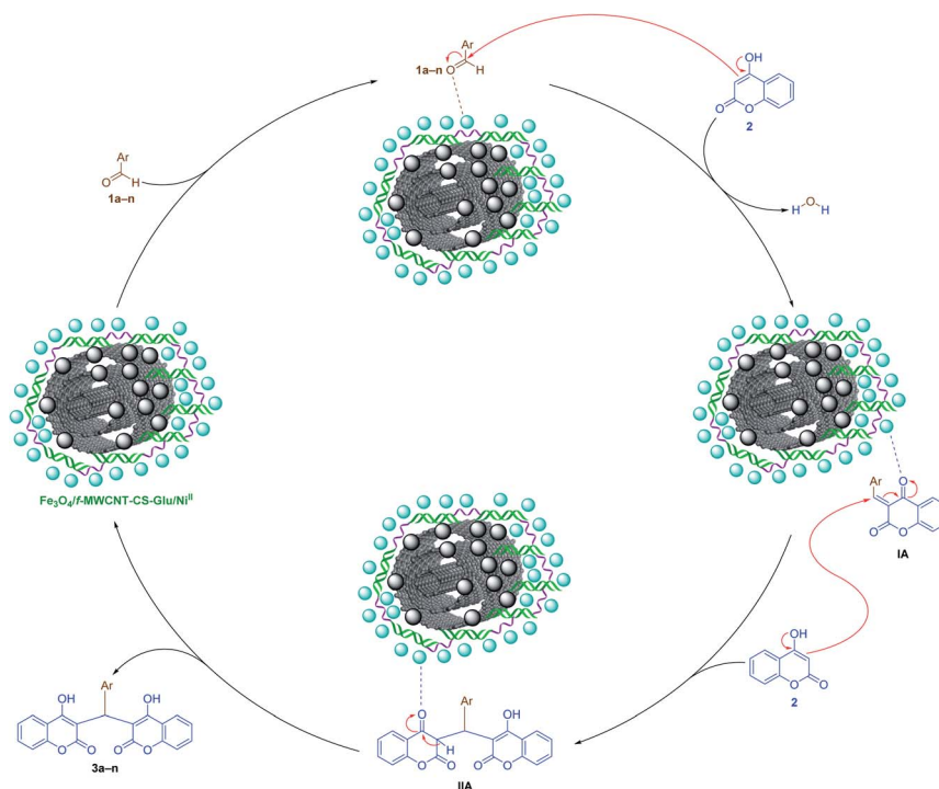
Scheme 3 Plausible mechanism for the one-pot pseudo -three-component synthesis of bis-coumarins in the presence of the as-prepared \text{Fe}_3\text{O}_4/\text{f-MWCNT-CS-Glu/Ni}^{\text{II}} nanocatalyst.
