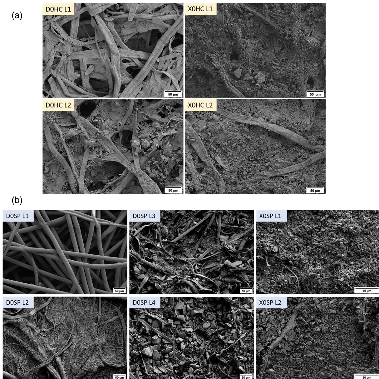
FIGURE 2 (a) Scanning electron microscopy images of the cellulose and DE-based Millistak+ D0HC (primary) and X0HC (secondary). (b) Scanning electron microscopy images of the synthetic based Millistak+ D0SP (primary) and X0SP (secondary)
