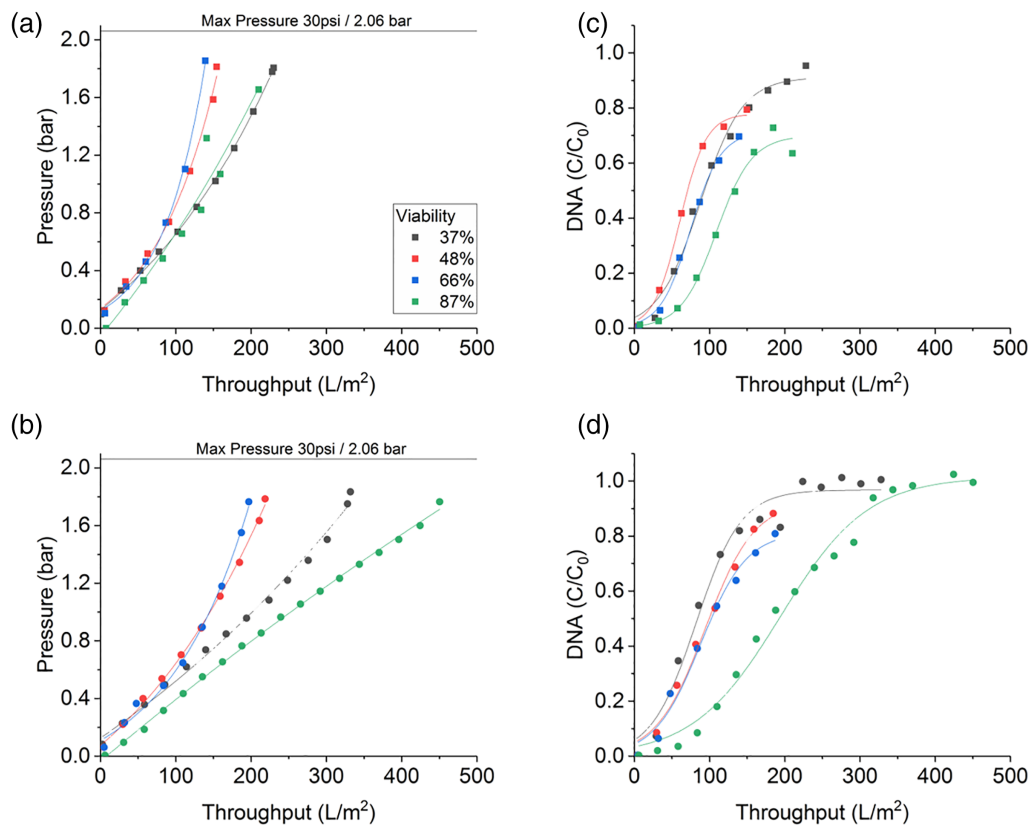
FIGURE 6 Pressure profile of secondary filters X0HC (a) and XOSP (b) as a function of volumetric throughput, and corresponding DNA breakthrough after secondary X0HC (c) and XOSP (d) using cell culture at different viability described in Table 1. Throughput was adjusted for the hold-up volume of the filters
