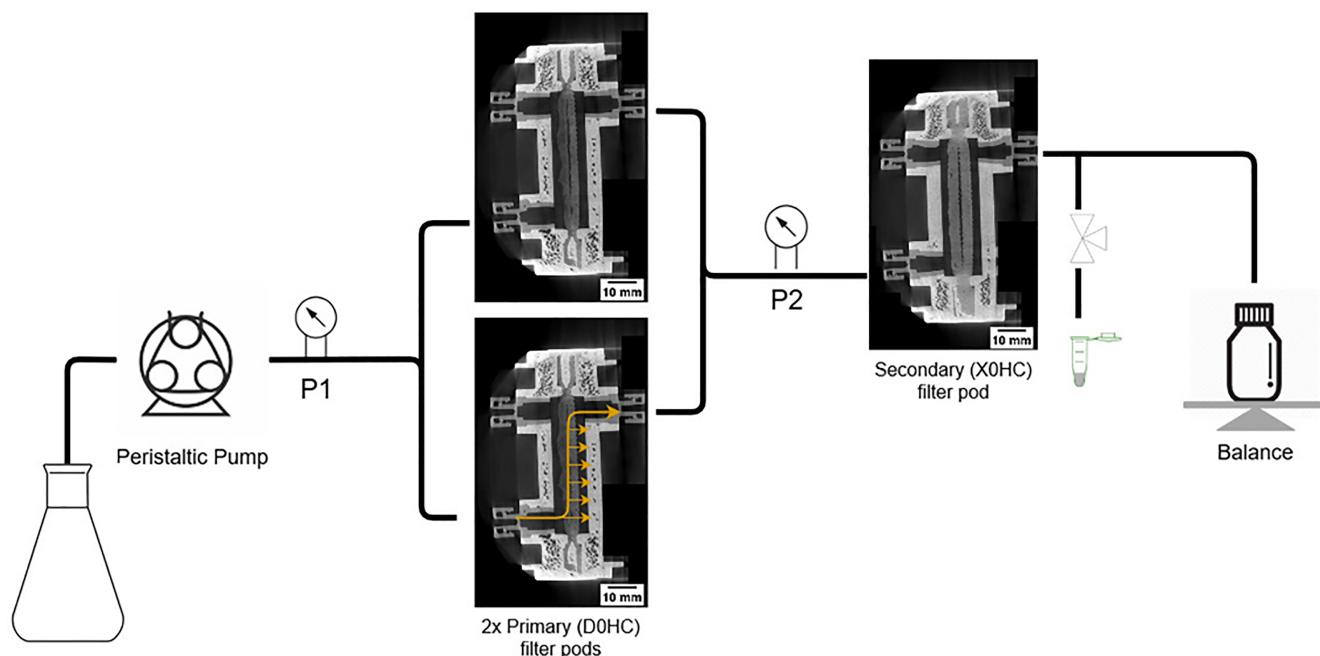
FIGURE 1 Schematic of depth filtration scale down model, with CT X-ray cross-section images of Millipore Millistak+ \mu Pods DOHC (primary) and X0HC (secondary). The yellow arrow indicates the direction of flow in the filter pods
