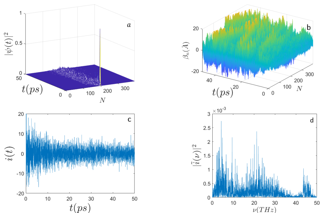
Figure 4. Time evolution of (a) the electron probability amplitude |\Psi(t)|^2 ; (b) the average displacements \beta_n (Å); (c) the electron current i(t) (expressed in \mu\text{biot} ); (d) the frequency spectrum |\tilde{i}(\nu)|^2 along the sequence of N = 398 nucleotides with the initial condition E_0 = 0.46 eV ( E' = 70 ). The initial electron excitation peaks around the site n_0 = N/2 . The other parameters are the same as those in Figure 1.
