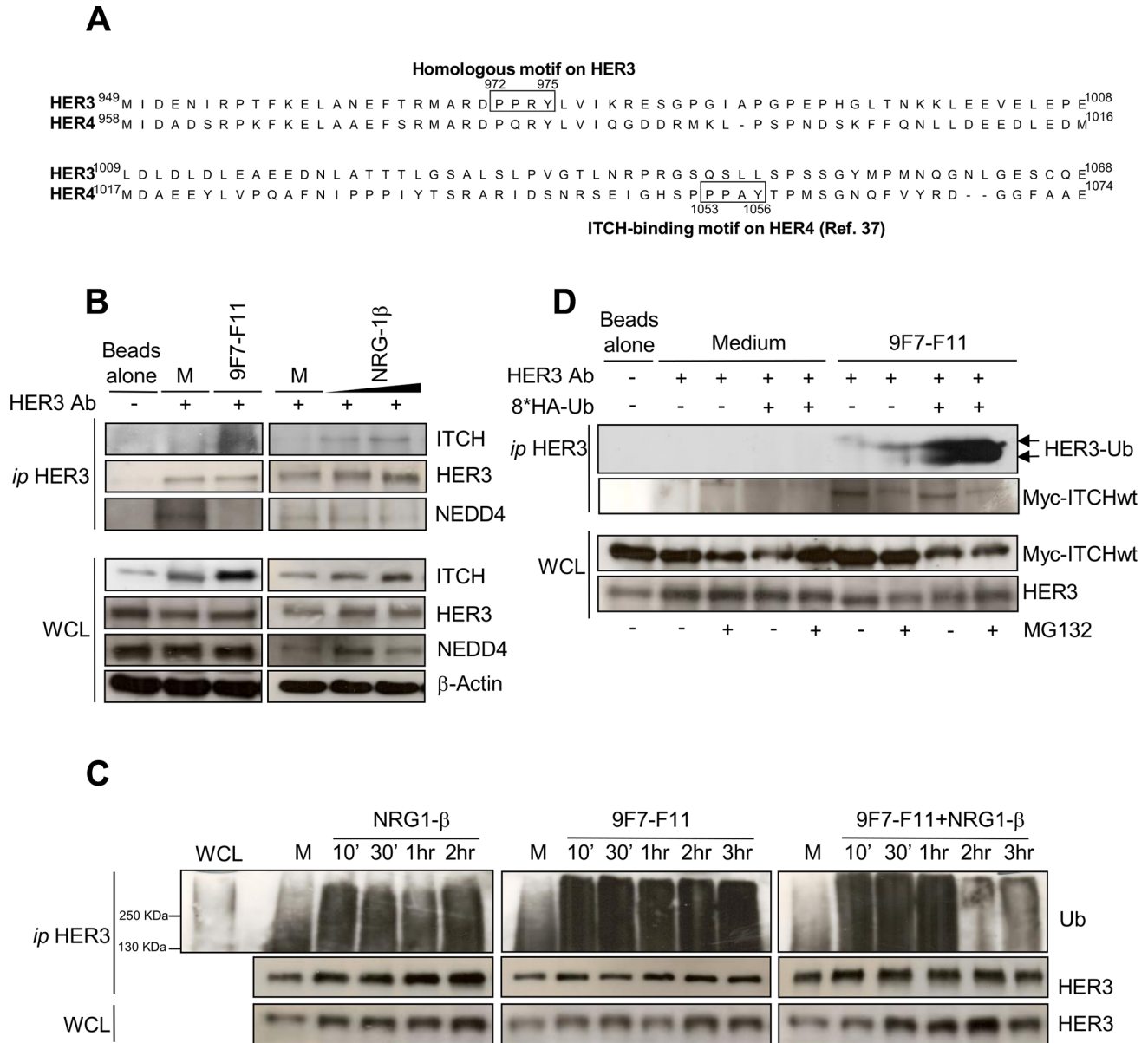
Figure 4: ITCH interacts with HER3 and the anti-HER3 antibody 9F7-F11 induces ITCH recruitment leading to HER3 ubiquitination and disruption of NEDD4/HER3 interaction. (A) Protein sequence alignment of HER3 and HER4 C-terminal tails showing the homology between the HER3 972 PPRY 975 motif and the ITCH-binding motif 1053 PPAY 1056 in HER4. (B) Serum-starved BxPC3 cells were incubated with 50 \mu g/mL 9F7-F11 for 30 min or with 100ng/mL NRG-1 \beta for 30 min or 1 hr. After immunoprecipitation (ip) of 2 mg of total protein extracts with an anti-HER3 monoclonal antibody against HER3 C-terminal tail (HER3 Ab), ITCH, HER3 and NEDD4 were detected by western blotting. (C) Serum-starved BxPC3 cells were pre-incubated with 10 \mu M MG132 for 4 hr before incubation with 50 \mu g/mL 9F7-F11 with or without 100 ng/mL NRG-1 \beta for the indicated times. After immunoprecipitation with HER3 Ab, HER3 ubiquitination status was assessed by western blotting using a specific anti-ubiquitin antibody (Ub). (D) MDA-MB468 cells were transfected with the Myc-ITCH plasmid and the HA-Ubiquitin plasmid or not for 24 hr. Then, cells were incubated with 20 \mu M MG132 for 5 hr before addition of 50 \mu g/mL 9F7-F11 for 2 hr. After immunoprecipitation with HER3 Ab, HER3 was probed with an ubiquitin-specific antibody as in (C). WCL, whole cell lysate.
