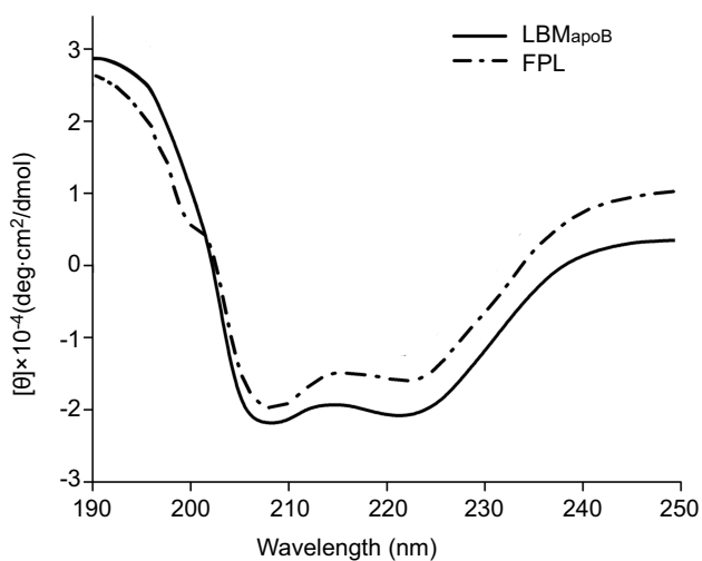
Figure 2 CD spectra of \text{LBM}_{\text{apoB}} and FPL peptides in trifluoroethanol. Abbreviations: CD, circular dichroism; FPL, FA-PEG- \text{LBM}_{\text{apoB}} ; \text{LBM}_{\text{apoB}} , lipid-binding motif of apoB-100.
