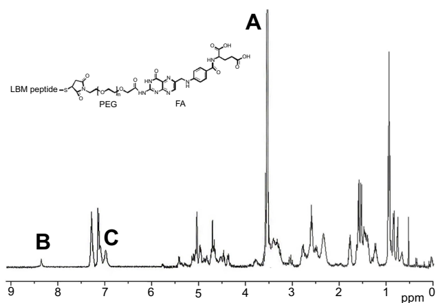
Figure 1 ^1\text{H} NMR spectrum of FPL hybrid peptide (A) the characteristic peak of PEG; (B) the characteristic peak of FA; (C) the characteristic peak of \text{LBM}_{\text{apoB}} . Abbreviations: FPL, FA-PEG- \text{LBM}_{\text{apoB}} ; FA, folic acid; \text{LBM}_{\text{apoB}} , lipid-binding motif of apoB-100.
