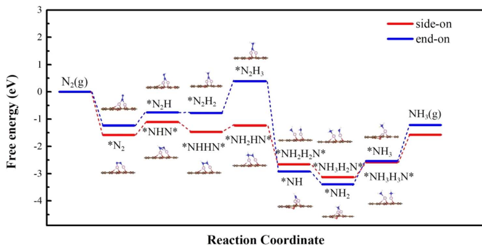
Fig. 7 Free energy diagram along the reaction path of NRR proceeded on O-CoCo-O starting with side-on and end-on configuration.
