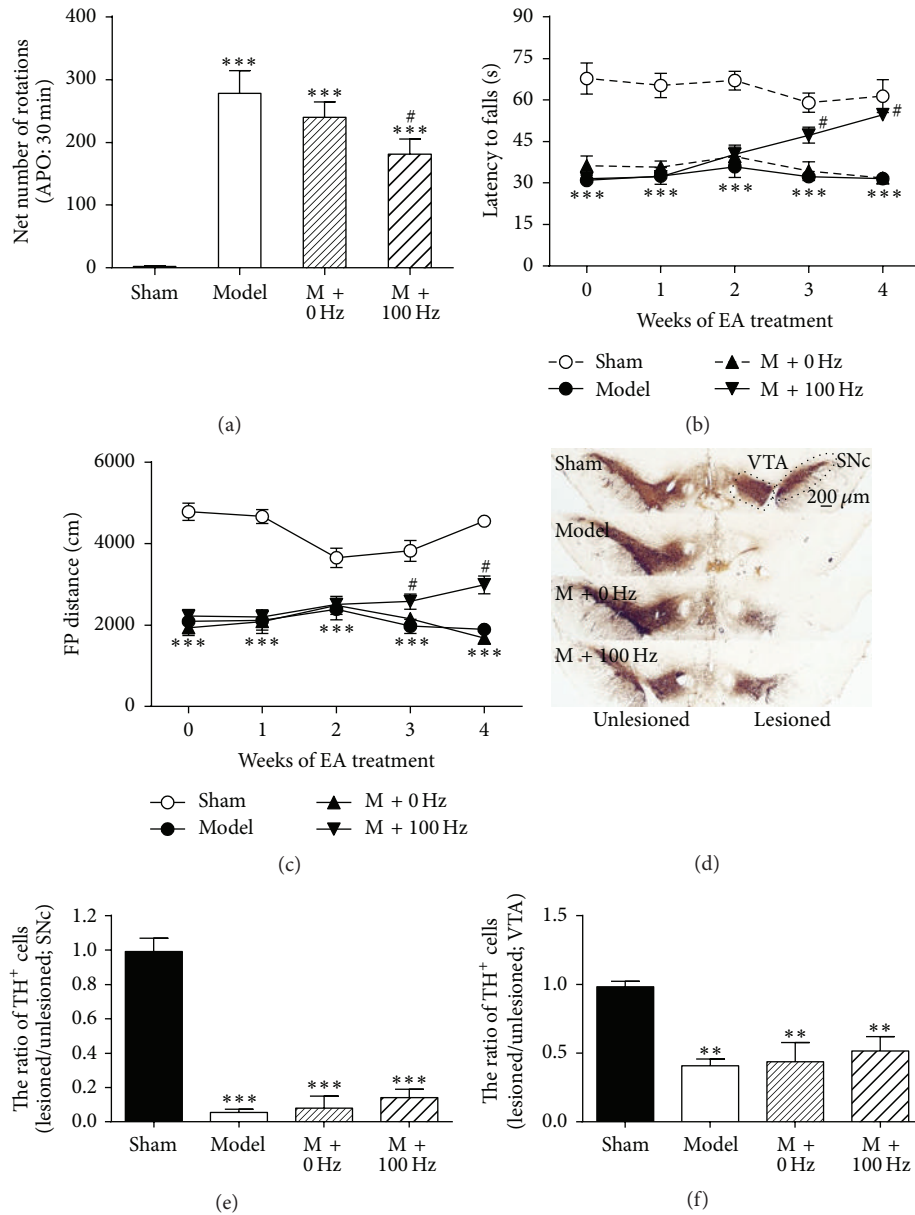
FIGURE 1: Effects of 100 Hz EA treatment on motor symptoms and dopaminergic neurodegeneration in the ventral midbrain of 6-OHDA lesioned rats. ((a)–(c)) Effects of EA on APO-induced rotational behavior (a), rotarod test (b), and horizontal movement distance in the open field test (c). Data represent mean \pm SEM ( n = 9 –11 per group). ** P < 0.01 and *** P < 0.001 versus the sham group; # P < 0.05 versus the model group. (d) Effects of EA on TH immunohistochemical staining. SNc is implied by the elliptical dotted line and VTA is implied by rectangle dotted line in (d). ((e) and (f)) Quantification of the damaged extent of TH-positive profiles on lesioned compared to unlesioned side in the SNc (e) and in the VTA (f). Data represent mean \pm SEM, ** P < 0.01 , and *** P < 0.001 versus the sham group.
