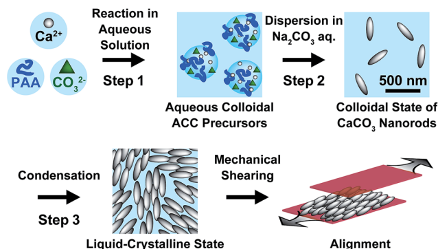
Fig. 1 Synthetic approach and alignment control for liquid-crystalline CaCO 3 .
