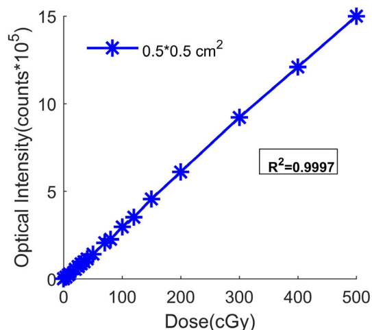
FIG. 4. Inorganic scintillator detector signal linearity with dose. [Color figure can be viewed at wileyonlinelibrary.com ]
