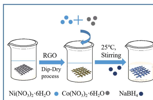
Fig. 1 The schematic diagram of the preparation process of Co–Ni–B/RGO/cotton fabric composite electrode.
