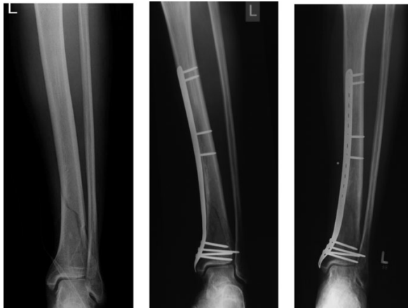
Figure 6. Example of a dynamic plate osteosynthesis in a distal tibial fracture. Preoperative (left), postoperative (middle), and radiographs after fracture healing (right) are shown. A long plate with a limited number of screws is used. Screws close to the fracture site and lag screws are avoided.
