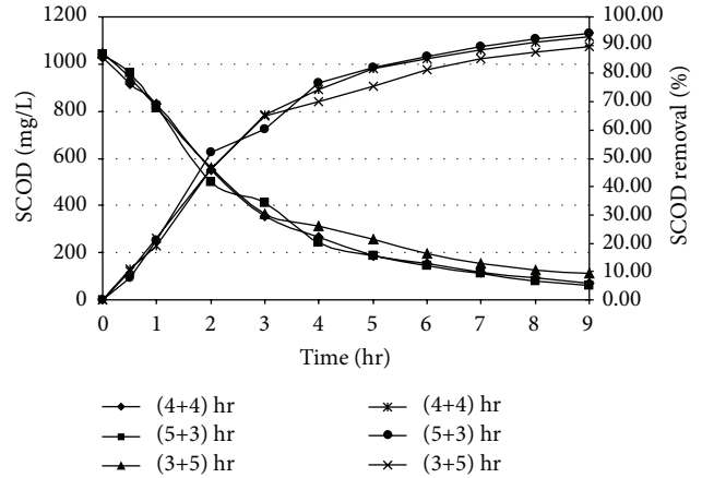
FIGURE 3: Carbon oxidation profile in SBR under different react period combination [Initial SCOD = 1000 ± 50 mg/L; Initial NH 4 + -N = 180 ± 10 mg/L as N].
