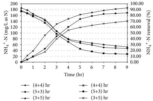
FIGURE 5: Ammonia oxidation profile in SBR under different react period combination [Initial SCOD = 1000 \pm 50 mg/L; Initial \text{NH}_4^+ -N = 180 \pm 10 mg/L as N].
