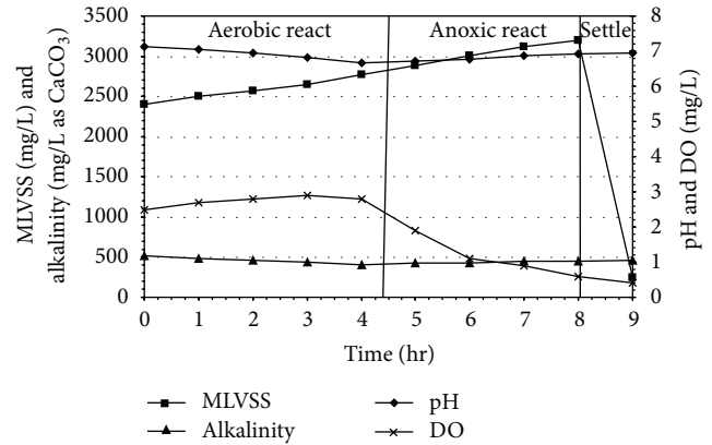
FIGURE 8: MLVSS, pH, alkalinity, and DO profiles for slaughterhouse wastewater treatment in SBR under (4+4) hr react period combination.
