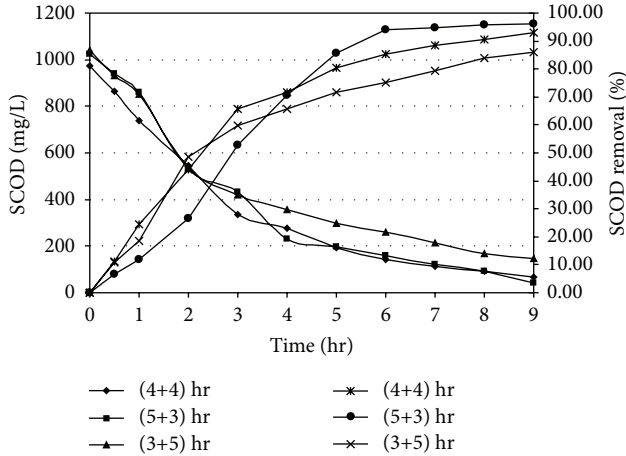
FIGURE 2: Carbon oxidation profile under different react period combination [Initial SCOD = 1000 ± 50 mg/L; Initial NH 4 + -N = 90 ± 10 mg/L as N].
