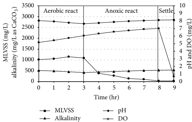
FIGURE 10: MLVSS, pH, alkalinity, and DO profiles for slaughterhouse wastewater treatment in SBR under (3+5) hr react period combination.
