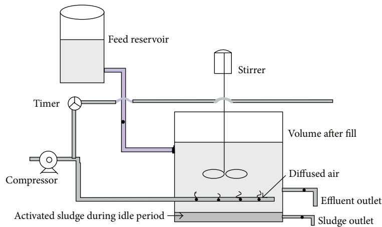
FIGURE 1: A schematic diagram of the experimental setup.
