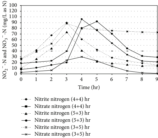
FIGURE 7: Nitrite and nitrate concentration profiles in SBR under different react period combination [initial SCOD = 1000 ± 50 mg/L and initial NH 4 + -N = 180 ± 10 mg/L as N].
