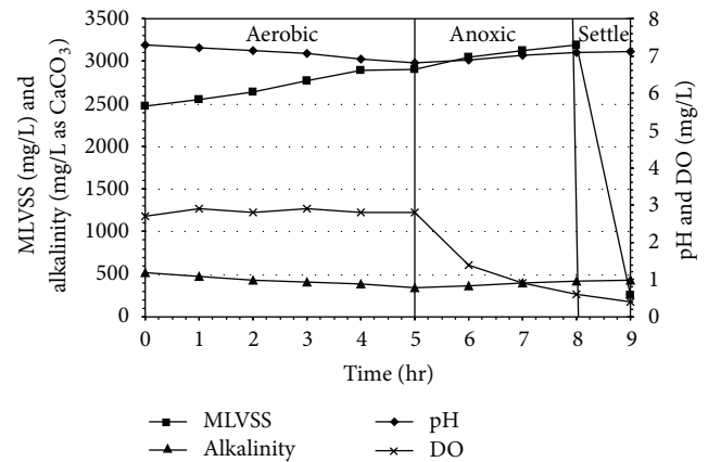
FIGURE 9: MLVSS, pH, alkalinity, and DO profiles for slaughterhouse wastewater treatment in SBR under (5+3) hr react period combination.
