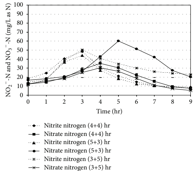
FIGURE 6: Nitrite and nitrate concentration profiles in SBR under different react period combination [initial SCOD = 1000 \pm 50 mg/L and initial \text{NH}_4^+ -N = 90 \pm 10 mg/L as N].
