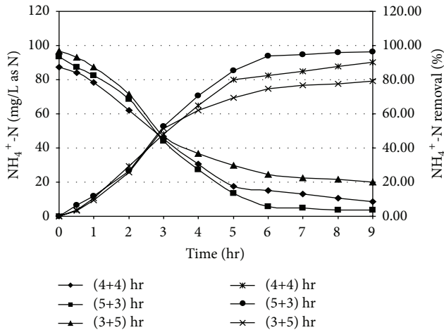
FIGURE 4: Ammonia oxidation profile in SBR under different react period combination [Initial SCOD = 1000 \pm 50 mg/L; Initial \text{NH}_4^+ -N = 90 \pm 10 mg/L as N].
