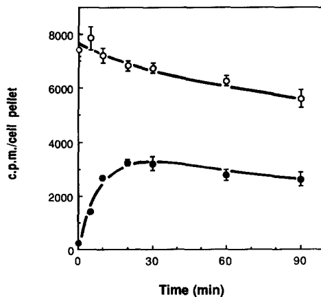
Figure 2. CD4 endocytosis on HL-60 cells. CD4 was traced on HL-60 cells using ^{125}\text{I} -4120 antibody (0.6 nM). After warming ^{125}\text{I} -4120-labeled cells for various times, levels of total cell-associated (○) or low pH-resistant activity (●) were determined by acid washing and \gamma -counting. Error bars indicate standard deviations for measurements from triplicate cell samples.
