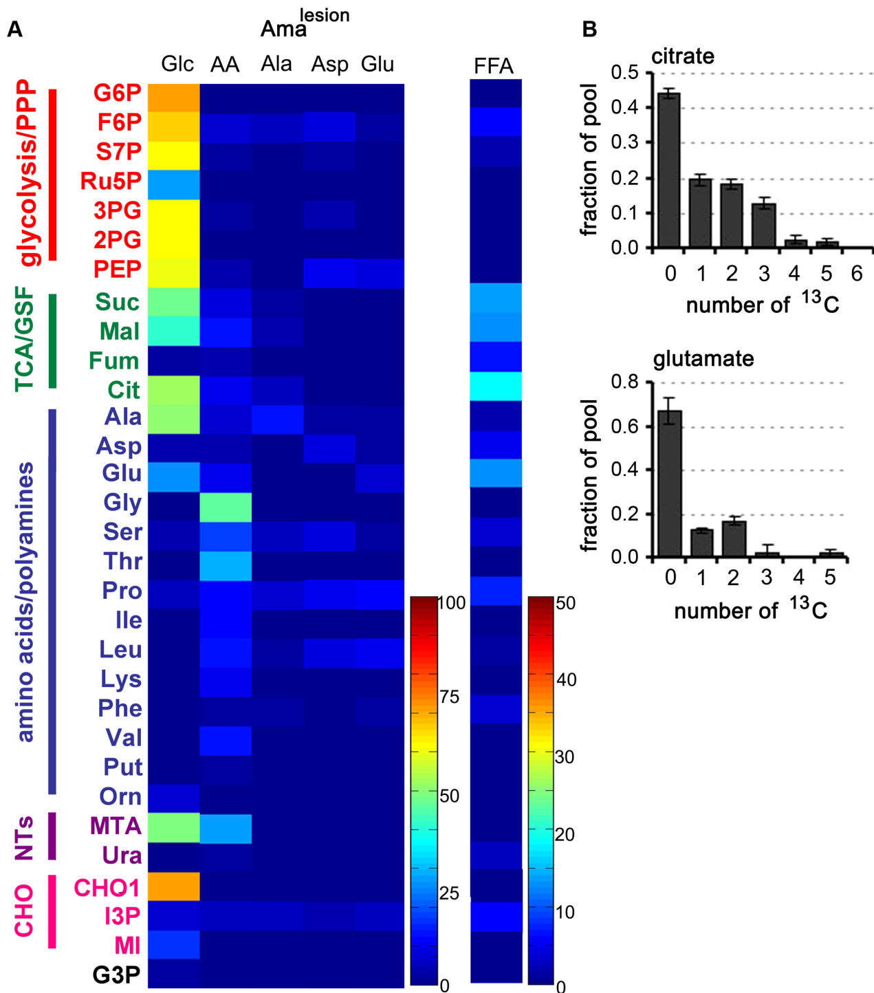
Figure 5. Carbon source utilization by Ama lesion . A. L. mexicana amastigotes were harvested from susceptible Balb/c mice lesions and purified Ama lesion immediately suspended in CDM containing either ^{13}\text{C} -U-glucose (Glc), a mixture of ^{13}\text{C} -U-amino acids (AA), ^{13}\text{C} -U-alanine (Ala), ^{13}\text{C} -U-aspartate (Asp), ^{13}\text{C} -U-glutamate (Glu), or ^{13}\text{C} -U-fatty acids (FFA). Isotopic enrichment in intracellular pools of metabolites in central carbon metabolism was determined by GC-MS (see also Tables S1–S7 in Text S1). B. The uptake of ^{13}\text{C} -U-glucose and the secretion of labeled end products in Ama lesion were determined by ^{13}\text{C} -NMR analysis of culture supernatant after 24 h incubation. C. Mass isotopomer of citrate and glutamate in Ama lesion labelled with ^{13}\text{C} -U-fatty acids for 3 h. Data represent mean (n=3) and SD. doi:10.1371/journal.ppat.1003888.g005
