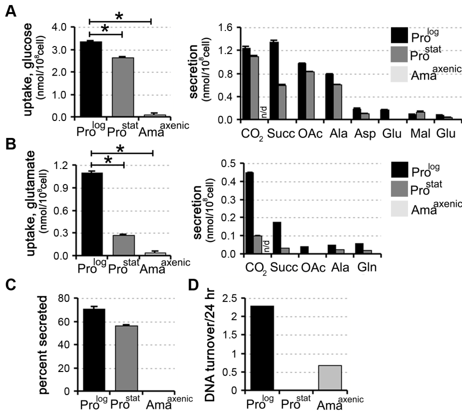
Figure 1. Carbon source utilization by different L. mexicana developmental stages. L. mexicana Pro log , Pro stat and Ama axenic were suspended in chemically defined medium (CDM) containing ^{13}\text{C} -U-glucose (A) or ^{13}\text{C} -glutamate (B) and the rate of utilization of the proffered ^{13}\text{C} -carbon source (left hand panel) and production of overflow metabolites (right hand panel) assessed by ^{13}\text{C} -NMR analysis of the conditioned medium. ^{13}\text{CO}_2 (detected as \text{H}^{13}\text{CO}_3^- ) was only quantified in the medium of promastigote stages, as it is not retained in the acidified amastigote medium. C. Proportion of internalized ^{13}\text{C} -glucose that was secreted as partially oxidized end-products by Pro log , Pro stat and Ama axenic . Similar relative levels of secretion were observed in the two promastigote stages (~50%), while negligible secretion was observed in Ama axenic . D. Replication rates of different L. mexicana developmental stages. Pro log , Pro stat and Ama axenic were cultivated in RPMI supplemented with \text{D}_2\text{O} (5% v/v, final) and the rate of DNA turnover determined by kinetic analysis of deuterium incorporation into adenosine deoxyribose. All data represent mean ( n=3 ) and standard deviation and are representative of several independent experiments. doi:10.1371/journal.ppat.1003888.g001
