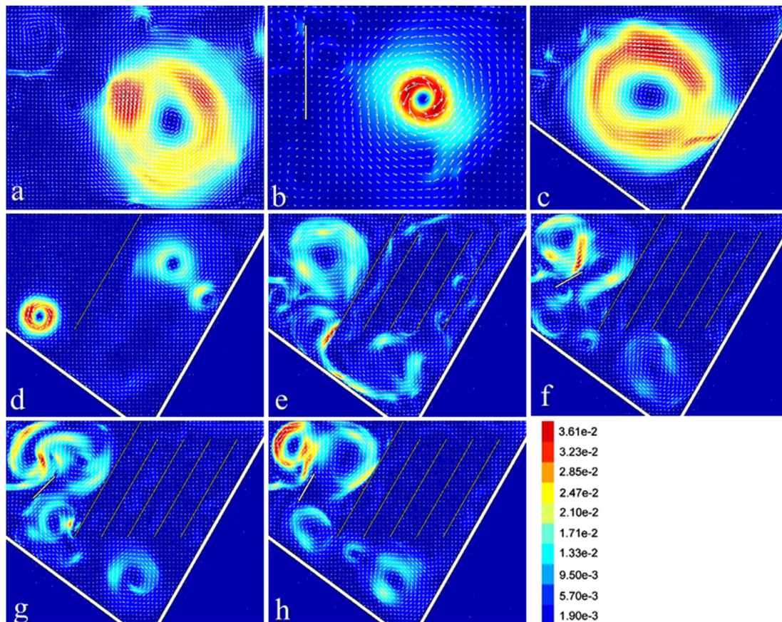
Figure 4. Kinetic energy (J kg -1 ) and velocity field for the different geometries. Each frame is 0.6 m tall and 0.68 m long. Letters (a–h) correspond to configurations shown in Figure 1.
