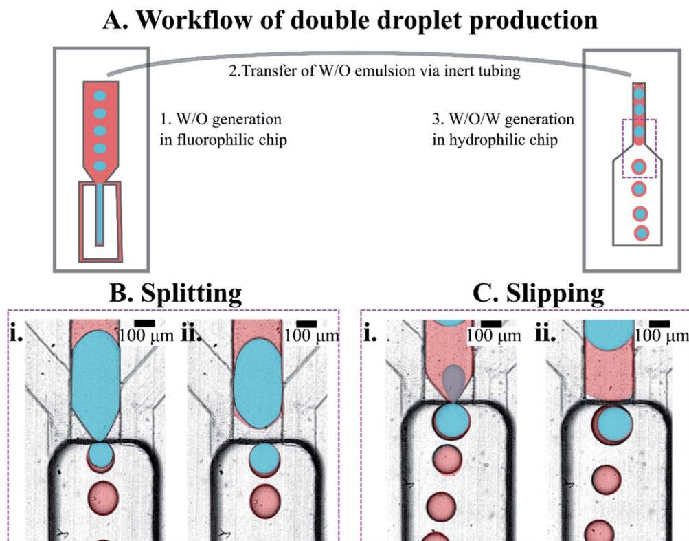
Fig. 4 Generation of double emulsion droplets using tandem step microfluidics. (A) Workflow of the production of the double droplets. (B and C) Magnification of area where droplets are formed. Snapshots from the step emulsification experiments – in each, the frames (i) and (ii) were taken a few milliseconds apart. Two observed behaviors of the core droplets during DE production on a step. Either the core droplet split into multiple droplets ((B), two panels in the left) or slipped whole to the DE ((C), two panels in the right). Core droplets in splitting regime (B) are made of PVA 2% wt, core droplets in slipping regime (C) are made of PVA 10% wt. Water phase is colored blue in the image, but is transparent in reality; oil phase – red in the image, transparent in reality; outer phase – transparent both in image and in reality. Colors were added for clarity in the post-processing of the image.
