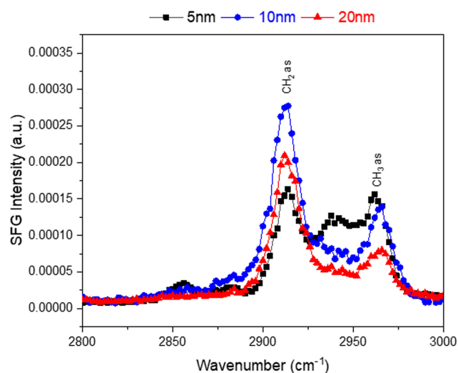
Figure 5 SFG spectra showing the CH region for each of the 5, 10, 20 nm Au-SOA-NP-coated HT. The NPs are at an air/water interface free of any lipids. The CH 2 asymmetric stretch is at 2913 cm -1 with the CH 3 asymmetric stretch at 2963 cm -1 . The NPs exhibit only asymmetric stretches which indicates strong ordering of the lipid coating.
