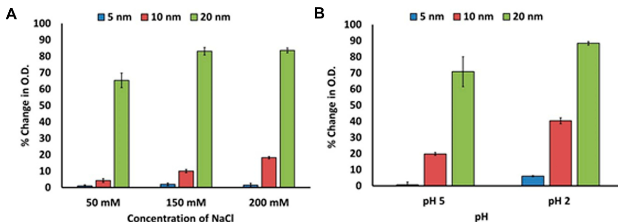
Figure 2 Percent change in O.D. of hybrid lipid capped Au-SOA-HPC-HT in 10 mM sodium phosphate buffer pH 8.0 | h after (A) exposure to 50 mM, 150 mM, or 200 mM NaCl (aq) and (B) adjustment of pH to 2 and 5 with 2 M HCl. Data mean \pm SE reported for n = 3 .
