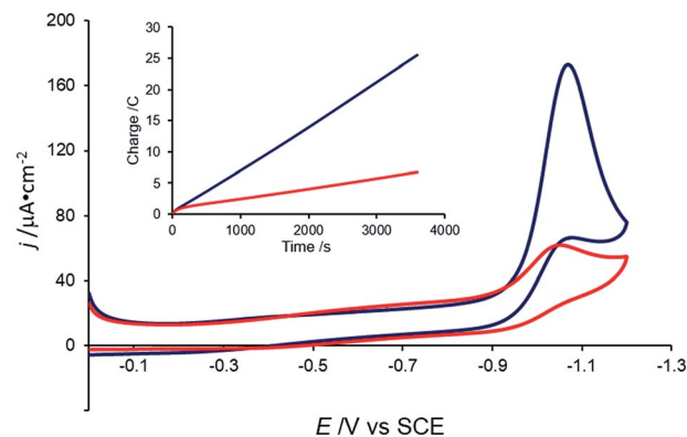
Fig. 7 Cyclic voltammogram of 0.5 mM [\text{Co}(\text{DIM})\text{Br}_2]^{+} with no \text{NaNO}_3 (red) and 10 mM \text{NaNO}_3 (blue) at pH = 4.6. Scan rate = 5 mV s -1 . Electrolyte: 50 mM KBr. Working electrode: GC. Inset: charge passed during CPE of 0.1 M \text{NaNO}_3 without catalyst (red) and with 0.5 mM [\text{Co}(\text{DIM})\text{Br}_2]^{+} (blue). Carbon rod electrode. Initial pH = 3.5.
