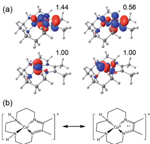
Fig. 6 (a) Calculated NOs (isovalue = 0.05 e \text{ \AA}^{-3} ) of the AF-triplet state of [\text{Co}(\text{DIM})]^{+} . The occupation numbers of each NO are indicated. (b) A scheme showing how this electronic structure can be described in terms of resonance structures and formal oxidation states.
