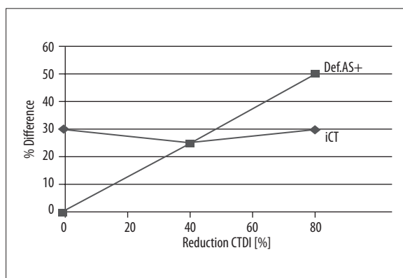
Figure 3. Correlation between reduction of CTDI vol and relative difference in low contrast (LC): % difference = \emptyset_{\min}(\text{FBP}) - \emptyset_{\min}(\text{IR}) / \emptyset_{\min}(\text{FBP}) [%]. Reduction of CTDI = \text{MaxCTDI} - \text{CTDI}(i) / \text{MaxCTDI} [%].
