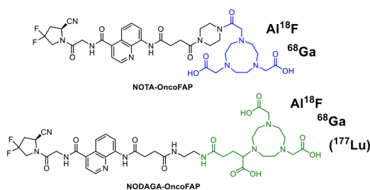
Fig. 4 FAP \alpha -conjugates for hybrid radiolabelling using radiometals and the \text{Al}^{18}\text{F} technique.
