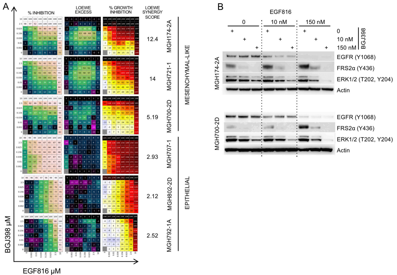
Figure 2. FGFR inhibition synergizes with EGFR TKI in mesenchymal, EGFR TKI-resistant cell lines.
