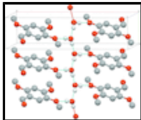
Fig. 2. Partial packing view showing the polymeric chains extending along the b axis.
