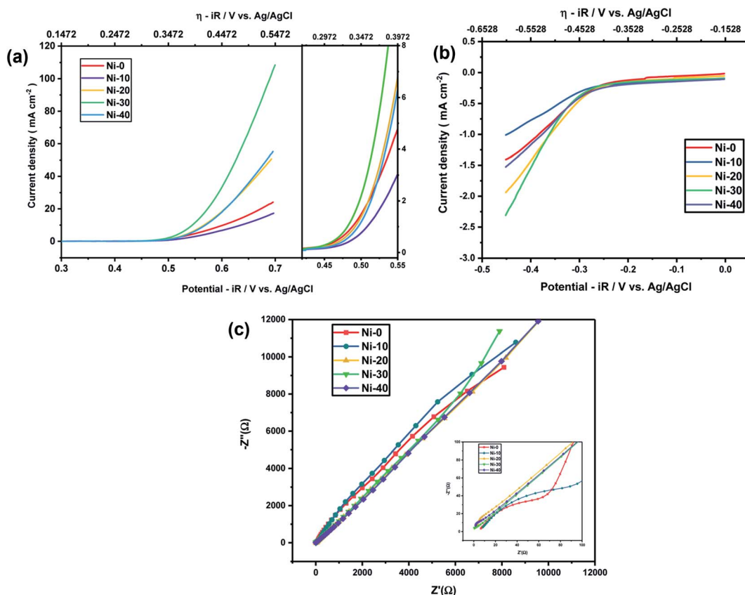
Fig. 6 (a) OER activity of \text{Ni}_x\text{Co}_{1-x}\text{O} at 5 M KOH electrolyte. (b) ORR activity of \text{Ni}_x\text{Co}_{1-x}\text{O} at 5 M KOH electrolyte. (c) EIS measurements of \text{Ni}_x\text{Co}_{1-x}\text{O} at 5 M KOH electrolyte.
