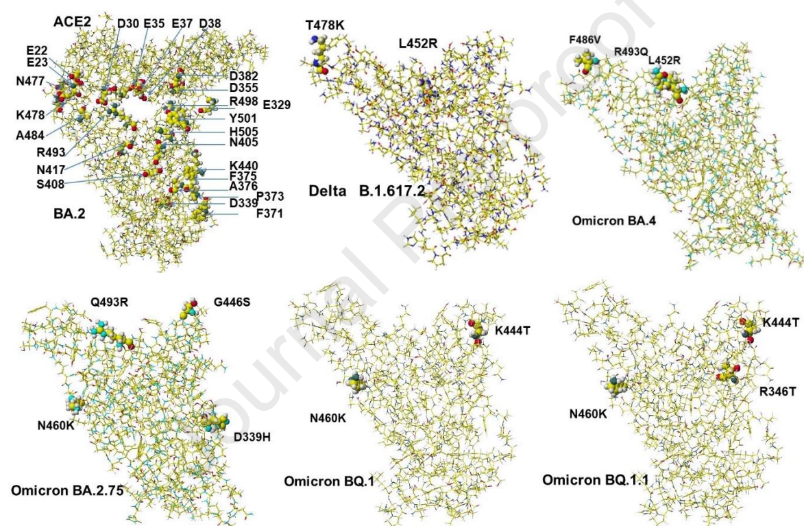
Figure 1. Structure of ACE-2 complexes with S-RBD of Delta, Omicron BA.2 with ACE-2, BA.2.75, BA.4 (BA.5), BQ.1 and BQ.1.1.
