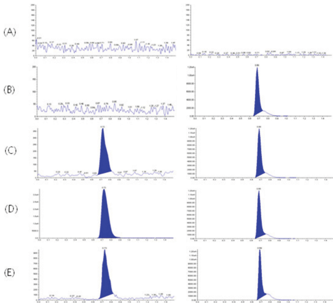
Supplementary Fig. 1. Representative chromatograms for selected extracted samples (left for PT; right for IS) at double blank (A), blank sample (B), LLOQ (50 ng/mL, C), HLOQ (2,000 ng/mL, D), and real sample (E) in rat plasma.
