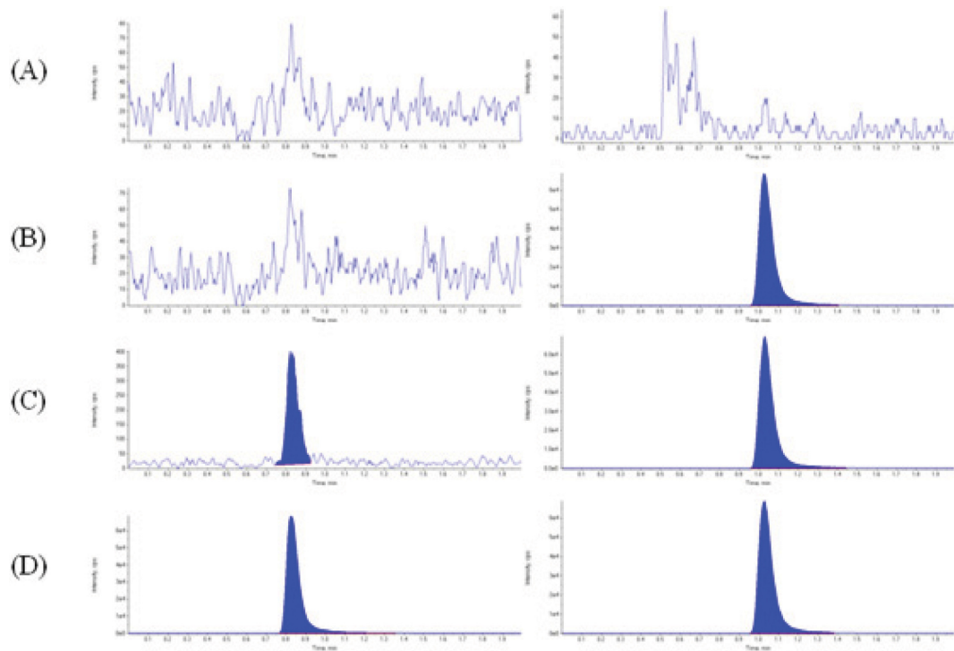
Supplementary Fig. 3. Representative chromatograms for selected extracted samples (left for MSP; right for IS) at double blank (A), blank sample (B), LLOQ (5 ng/mL, C), and HLOQ (1,000 ng/mL, D) in rat plasma.
