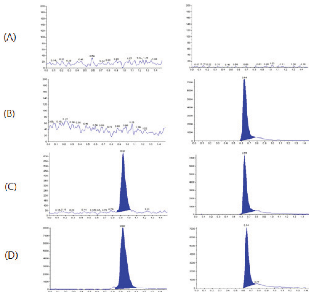
Supplementary Fig. 4. Representative chromatograms for selected extracted samples (left for ZnPT; right for IS) at double blank (A), blank sample (B), LLOQ (50 ng/mL, C), and HLOQ (2,000 ng/mL, D) in shampoo solution.
