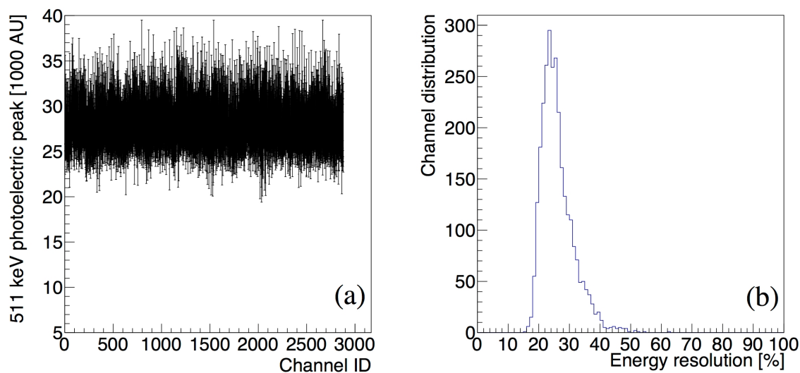
Figure 7. System calibration: position (ph pos ) (a) and energy resolution (FWHM/ph pos ) (b) of the 511 keV photoelectric peak measured during a 22 Na calibration run in the 2880 channels.
