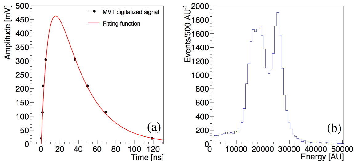
Figure 6. Response of a LYSO/SiPM channel after the detection of a 511 keV photon from a 22 Na source. In (a) the MVT digitalized signal (black points) and the fitted function reconstructing the original signal (red line) are shown. The fitted function is integrated within a time window of 200 ns and the distribution of its integral for a small sub-sample of 30,000 events is shown in (b): the photoelectric peak and the Compton continuum are visible in the obtained spectrum.
