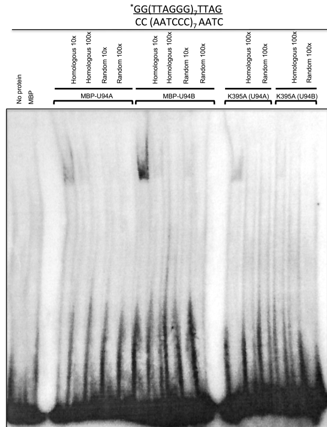
Figure 2. HHV-6 U94 binds double-stranded telomeric (TTAGGG/CCCTAA) probe. Proteins (MBP, MBP-Rep68, MBP-U94A, MBP-U94B and MBP-U94 K395A) were incubated with ^{32}\text{P} 5-end labeled probe for 30 min at 37°C in the absence or in the presence of identical or random competitor DNA. Loading dye was added to the samples and these were separated by electrophoresis on a non-denaturing gel. After migration the gel was dried and exposed to imaging plates. Results are representative of two independent experiments.
