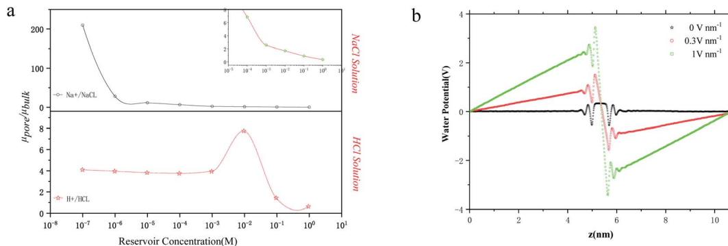
Fig. 4 Ion mobility and water potential for the sub-nm nanopore. (a) Ion mobility and ratio of ionic mobility inside the nanopore ( \mu_{\text{pore}} ) to the corresponding bulk mobility ( \mu_{\text{bulk}} ) as a function of reservoir concentration. The inset in the figure is a partial enlarged view of the \text{Na}^+ mobility, which shows that the change at low ionic concentration is still drastic. (b) Average axial electrostatic potential for \text{H}_2\text{O} in a MD model with a 2 nm nanopore for electric field strengths of 0 \text{ V nm}^{-1} , 0.3 \text{ V nm}^{-1} , and 0.5 \text{ V nm}^{-1} , respectively. The stronger the electric field, the stronger the ability to rearrange water molecules.
