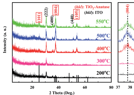
Fig. 2 XRD patterns of the \text{In}_{0.0025}\text{Nb}_{0.0025}\text{Ti}_{0.995}\text{O}_2 films on ITO/glass substrates annealing at 200 °C, 300 °C, 400 °C, 500 °C and 550 °C.
