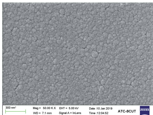
Fig. 3 SEM image of the \text{In}_{0.0025}\text{Nb}_{0.0025}\text{Ti}_{0.995}\text{O}_2 film on ITO/glass substrates annealed at 400 °C for 30 minutes.
