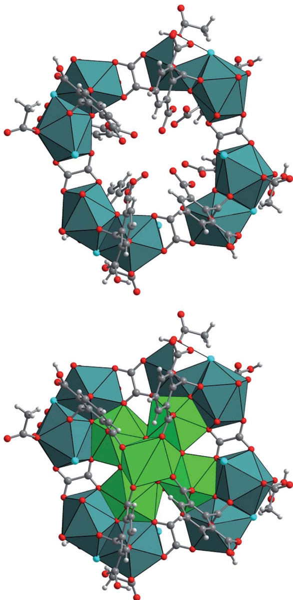
Fig. 6 (Top) Structure arrangement of the external crown-like [ U_8O_4Cl_4(ox)_4 ] ring composed of four dinuclear units (U3 and U4) that are further linked to each other via the oxalate molecules. (Bottom) Molecular structure of the poly-oxo cluster [ U_{14}O_8(OH)_4Cl_8(H_2O)_{16}(1,2,3-Hbtc)_8(ox)_4(ac)_4 ] (2). Green/slate circles and polyhedral; uranium, red circles; oxygen, grey circles; carbon, cyan circles; chlorine.
