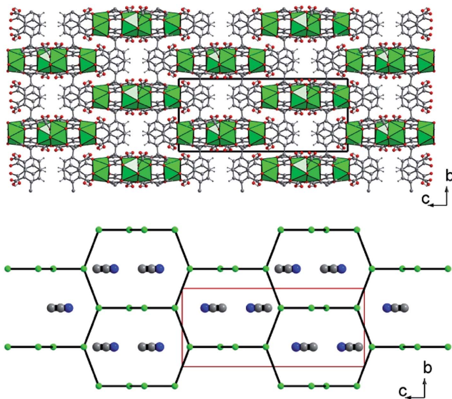
Fig. 3 (Top) Three-dimensional framework of U(1,2,3\text{-Hbtc})_2 \cdot 0.5\text{CH}_3\text{CN} ( 1 ). The blocks related to the four discrete \text{UO}_8 units correspond to the infinite corrugated ribbons shown in Fig. 2. (Bottom) Schematic representation of the three-dimensional network showing the channels developed along the a (or b ) axis, in which disordered acetonitrile species are encapsulated. The acetonitrile molecules are shown randomly due to their statistically disordered positions within the channels. Green polyhedral and circles; uranium, grey circles; carbon, blue circles; nitrogen (from acetonitrile).
