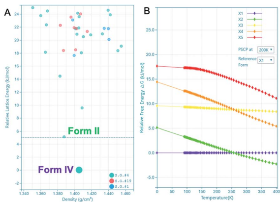
Fig. 6 CSP energy landscape of remdesivir (A) at 0 K and free energy profile of polymorphs (X1–X5) relative to X1 spanning a temperature range of 0 to 400 K (B). PSCP at 200 K refers to the free energy result obtained using the pseudo super critical path method with Einstein crystal of X1 at 200 K as the reference.
