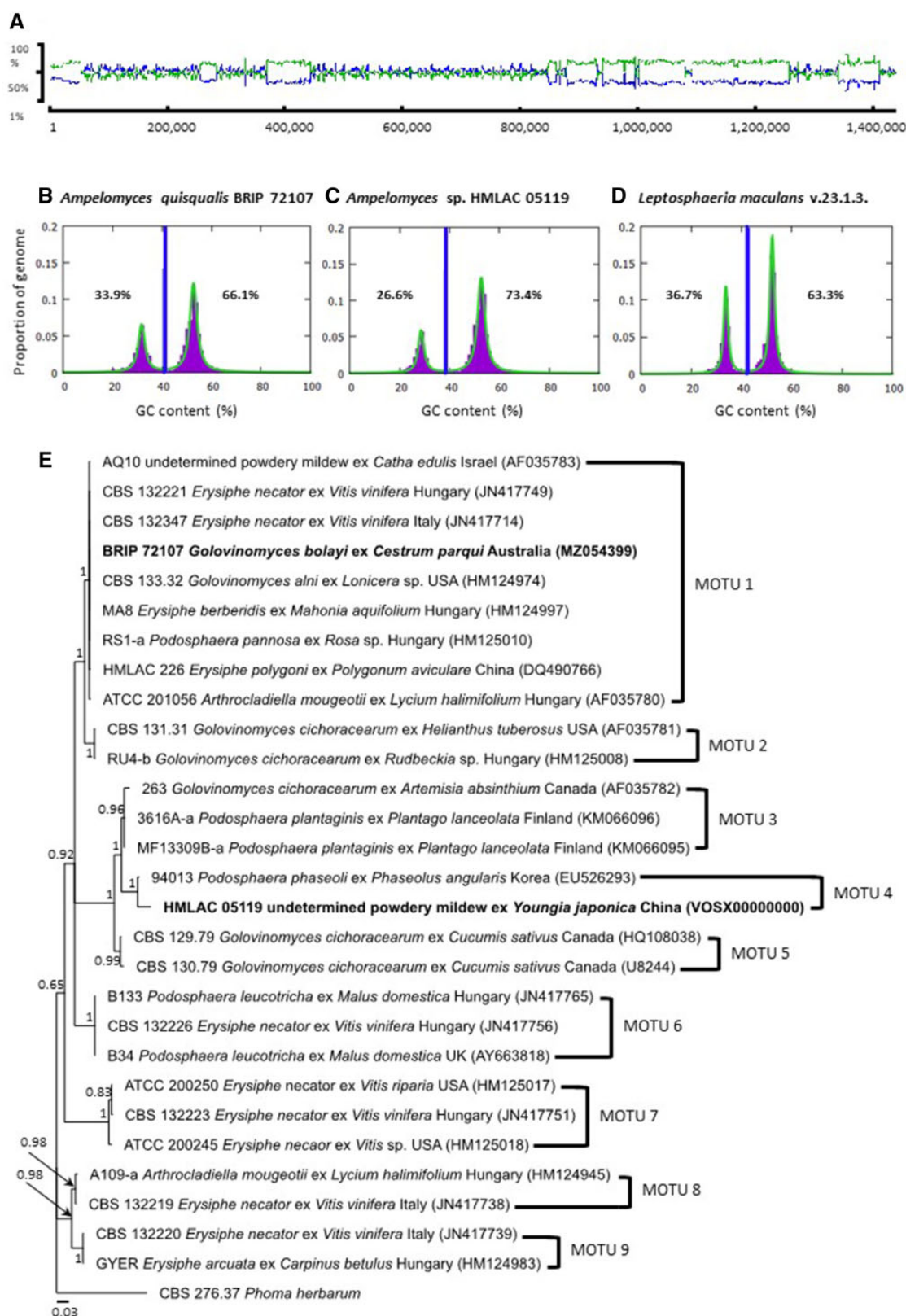
FIG. 1. —The first 1,400,000bp of BRIP 72107 contig-4 is demonstrated here as an example showing GC-balanced regions interspersed by longer or shorter stretches of AT-rich regions (A). The GC content distribution of Ampelomyces spp. (B and C) show striking similarity to the plant pathogenic fungus, Leptosphaeria maculans (D). Vertical blue lines show the GC cut-off points selected by OcculterCut (Testa et al. 2016) to classify genome segments into
