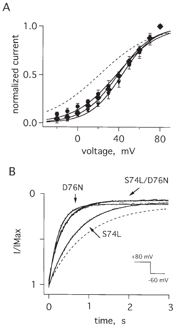
FIGURE 9. Gating attributes of mutant I_{Ks} channels. (A) Normalized open probabilities ( I/IMax ) for cells with D76N I_{Ks} channels ( \bullet , z = 1.3 \pm 0.2 ), S74L I_{Ks} channels ( \blacktriangledown , z = 1.6 \pm 0.1 ), and S74L-D76N I_{Ks} channels ( \blacklozenge , z = 1.3 \pm 0.2 ); protocols, theoretical fits, and equivalent valences ( z ) as in Fig. 5; the dotted line is the curve for wild-type I_{Ks} channels from Fig. 5 A. (B) Normalized tail currents at -60 mV for D76N, S74L, and D76N-S74L I_{Ks} channels; the dotted line is the curve for wild-type I_{Ks} channels from Fig. 5 B. Currents were elicited after a 6-s test pulse to 80 mV. Theoretical lines were constructed as described in the legend to Table I.
