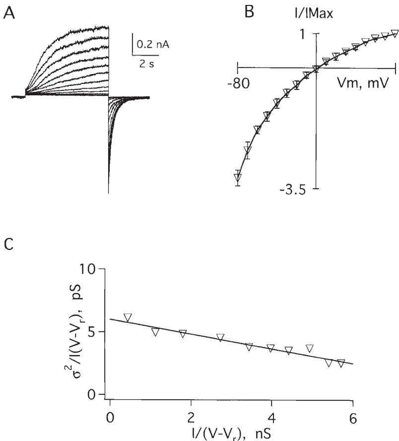
FIGURE 8. Current-variance relationships of I_{Ks} channels formed with S74L and D76N minK subunits. (A) Family of currents recorded from a patch excised from an oocyte coinjected with KvLQT1 cRNA and a 1:1 mixture of D76N and S74L minK cRNAs. The patch was clamped at -60 mV and depolarized from -20 to 100 mV in 10 -mV steps. (B) Current-voltage relationship of peak tail currents measured for channels, mean \pm SEM for three separate patches. (C) Current-variance relationship computed from the patch in A; the conductance calculated in this patch was 6.0 pS.
