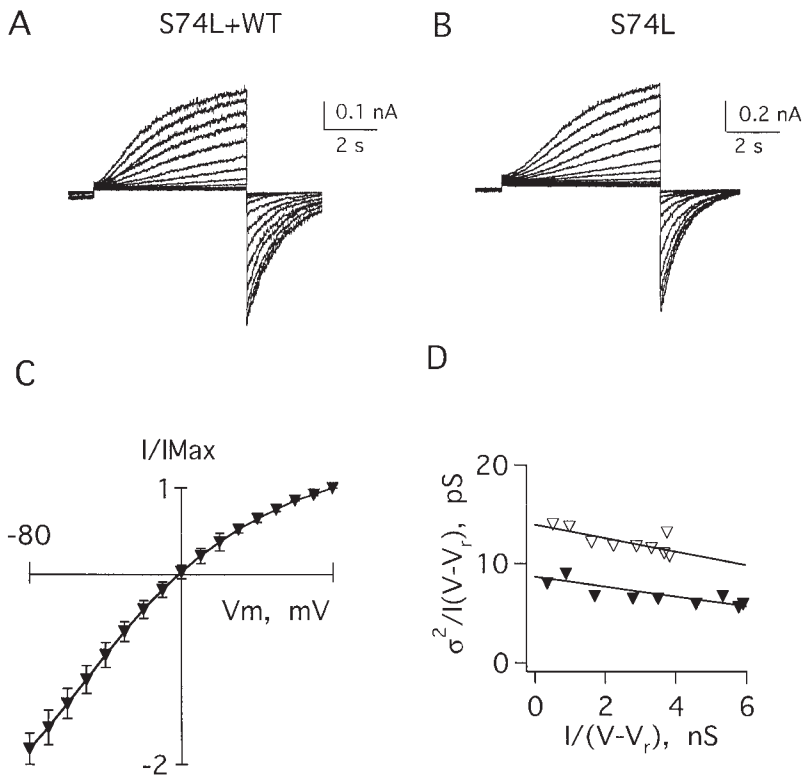
FIGURE 7. Current-variance relationships of I_{Ks} channels formed with wild-type and S74L minK subunits. (A) Family of currents recorded in a patch excised from an oocyte coinjected with KvLQT1 cRNA and a 1:1 mixture of wild-type and S74L minK cRNAs. The patch was clamped at -60 mV and depolarized from -20 to 100 mV in steps of 10 mV. (B) Family of currents recorded from oocytes coinjected only with KvLQT1 and S74L minK cRNAs. The protocol was as in A with steps from -20 to 90 mV. (C) Current-voltage relationship of peak tail currents measured for S74L I_{Ks} channels, mean \pm SEM for three patches. (D) Current-variance relationships computed from the patches in A ( \nabla ) and B ( \blacktriangledown ); the conductances calculated in these patches were 14 and 8.7 pS, respectively.
