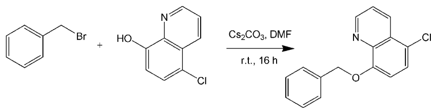
Scheme 3. Method for adding a linker arm to 5-chloro-8-hydroxyquinolone.
