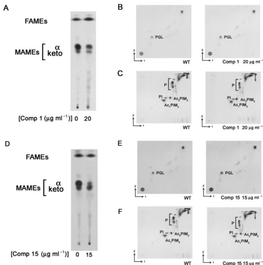
Fig. 3. TLC-autoradiography of M. bovis BCG lipids after NAS-21 and NAS-91 analogue treatment. (A, D) Analysis of FAMES and MAMES following treatment with NAS-21 analogue 1 (20 \mu\text{g ml}^{-1} ) and NAS-91 analogue 15 (15 \mu\text{g ml}^{-1} ) and resolved by TLC using equal counts (50 000 c.p.m.) as described in Methods. Lipid extractions were performed as described by Dobson et al. (1985) and a 50 000 c.p.m. aliquot analysed using silica gel plates (5735 silica gel 60F 254 ; Merck). (B, E) Phenolic glycolipids (PGL) were identified by 2D TLC [direction 1, chloroform/methanol (94:4, v/v); direction 2, toluene/acetone (80:20, v/v)]. (C, F) Phospholipids (P), phosphatidylinositol (PI), acyl-phosphatidylinositol dimannoside (Ac 1 PIM 2 ) and diacyl-phosphatidylinositol dimannoside (Ac 2 PIM 2 ) were identified by 2D TLC [direction 1, chloroform/methanol/water (60:30:6, by vol.); direction 2, chloroform/acetic acid/methanol/water (40:25:3:6, by vol.)]. Autoradiograms were produced by overnight exposure to Kodak X-Omat AR film to reveal 14 C-labelled FAMES, MAMES and lipids.
