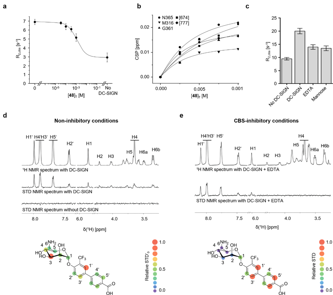
Figure 3. Ligand-observed binding mode analysis for DC-SIGN. (a) Titration experiments using the ^{19}\text{F} NMR RDA indicated interaction of 48 with DC-SIGNs CBS with affinity in the low millimolar range ( K_{\text{I}} = 1.15 \pm 0.01 mM). (b) The K_{\text{D}} value determined in ^{15}\text{N} HSQC NMR titrations indicated higher affinity than measured with the ^{19}\text{F} NMR RDA ( K_{\text{D}}, ^{15}\text{N} HSQC = 0.46 \pm 0.16 mM). (c) Direct ^{19}\text{F} R_2 -filtered NMR binding experiments using the trifluoromethyl group of 48 show incomplete inhibition in the presence of 4 mM EDTA or 200 mM mannose, suggesting a secondary \text{Ca}^{2+} -independent binding mode. (d) STD NMR experiments in the presence of \text{Ca}^{2+} served to determine the \text{Ca}^{2+} -dependent binding mode of 48 with DC-SIGN ECD. Specific STD effects were only observed in the presence of DC-SIGN ECD, allowing for epitopes to be determined from normalized \text{STD}'_0 values calculated from STD build-up curves at t_{\text{sat}} of 0.5, 1, 2, and 6 s (Figure S18). The STD NMR spectrum is magnified 4-fold. \text{STD}'_0 values in H3 and H4 indicated a mannose-type interaction with DC-SIGN, while a high \text{STD}'_0 in H1' suggested the -\text{CF}_3 on phenyl ring A to be involved in binding. (e) ^1\text{H} STD NMR experiments in the presence of EDTA- d_{11} served to validate the \text{Ca}^{2+} -independent binding mode with DC-SIGN ECD. Epitopes were obtained from normalized STD values calculated from STD spectra at t_{\text{sat}} of 2 s and displayed a shift from a mannose-dependent binding to an interaction dominated by the biphenyl-moiety in C1 in the absence of \text{Ca}^{2+} . The STD spectrum is magnified 4-fold. CBS-inhibition using an excess of mannose revealed similar STD NMR epitopes (Figure S19).
