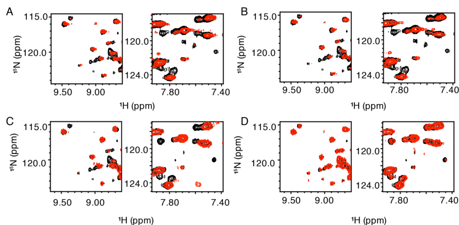
Figure 3. Effects of selected amino acids on the 2D ^1\text{H} – ^{15}\text{N} HSQC spectra of RDPHeH _{25-117} : 400 \mu\text{M} RDPHeH _{25-117} (black) and 400 \mu\text{M} RDPHeH _{25-117} (red) with (A) 10 mM D-phenylalanine, (B) 10 mM methionine, (C) 10 mM L-4-aminophenylalanine, and (D) 50 mM alanine. The two regions of the spectra shown are the same as those in Figure 2C. Conditions: 50 mM sodium phosphate, 100 mM NaCl, 1 \mu\text{M} leupeptin, 1 \mu\text{M} pepstatin A, and 10% D _2\text{O} (pH 8.0), at 300 K at a magnetic field strength of 11.7 T (500 MHz for ^1\text{H} ).
