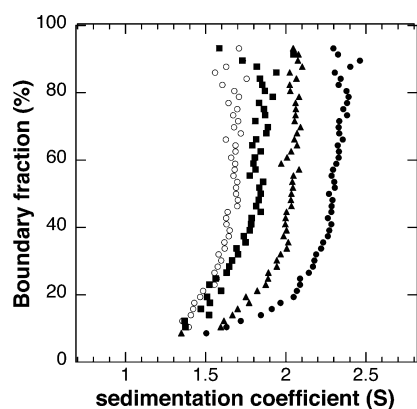
Figure 4. van Holde–Weischet distribution plot for RDPHeH _{25-117} ( \sim 15 \mu\text{M} total monomer) without (○) and with 50 mM leucine (■), 50 mM norleucine (▲), or 1 mM L-phenylalanine (●).
