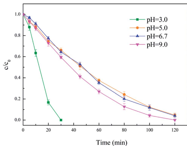
Fig. 8 Effect of initial pH. Conditions: 5% PTFE modified, I = 100 mA, catalyst 3 \text{ g L}^{-1} , 300 \text{ mL} diuron 10 \text{ mg L}^{-1} .
