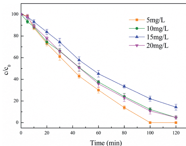
Fig. 9 Effect of diuron concentration. Conditions: 5% PTFE modified, I = 100 mA, catalyst 3 \text{ g L}^{-1} , \text{pH} 6.7 \pm 0.2 .
