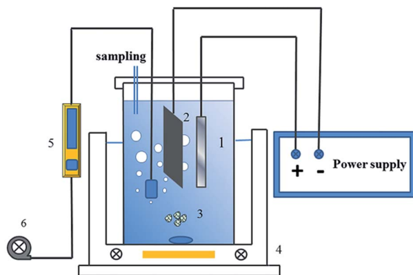
1. Anode 2. Cathode 3. Catalyst 4. Magnetic stirrer 5. Flowmeter 6. Aeration pump
