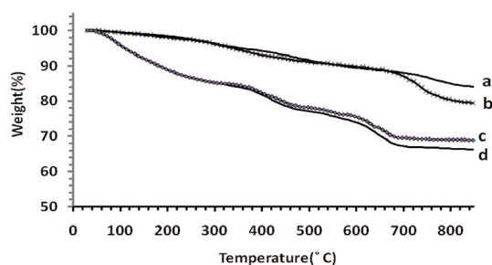
Fig. 2 TGA spectra of (a) Co@SiO 2 , (b) Co@SiO 2 -NH 2 , (c) Co@SiO 2 [(EtO) 3 Si-L 3 ]/Co(II) and (d) Mn@SiO 2 [(EtO) 3 Si-L 3 ]/Co(III).
