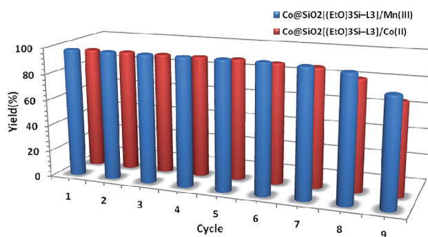
Fig. 9 Recycling of the two synthesized magnetic nanocatalysts used for the oxidation of methyl phenyl sulfide to methyl phenyl sulfoxide.
