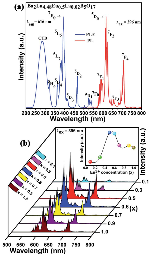
Fig. 3 (a) PLE ( \lambda_{em} = 616 nm) and PL ( \lambda_{ex} = 396 nm) spectra of Ba_2Lu_{4.48}Eu_{0.5}La_{0.02}B_5O_{17} ; (b) PL spectra for Ba_2Lu_{4.98-x}Eu_xLa_{0.02}B_5O_{17} ( x = 0.1, 0.3, 0.5, 0.6, 0.7, 0.9 and 1.0 ) phosphors. Inset shows the PL intensity as a function of Eu^{3+} concentration.
